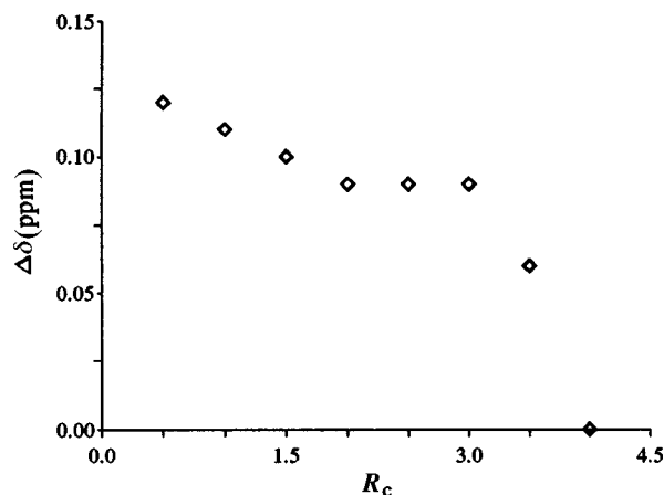
Fig. 4 \Delta\delta values relative to methyl protons as a function of R_c for the \text{Ag}(\text{I})\text{-Me}_2\text{Npe} system in \text{dms}\text{-d}_6 solution at 298 K. For free \text{Me}_2\text{Npe} \delta(\text{Me}) = 2.10 .
