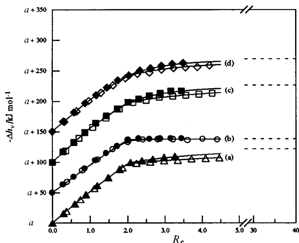
Fig. 2 The total molar enthalpy changes, \Delta h_v , as a function of R_c for silver(I)-P-N systems in dmso. (a) a = 0 for \text{Me}_2\text{Npe} : ( \Delta ) 2.075, ( \blacktriangle ) 6.977 \text{mmol dm}^{-3} in \text{Ag}^+ ; (b) a = -50 for \text{Me}_2\text{Npph} : ( \circ ) 1.892, ( \bullet ) 7.011 \text{mmol dm}^{-3} in \text{Ag}^+ ; (c) a = -100 for \text{Me}_2\text{Npp} : ( \square ) 1.953, ( \blacksquare ) 7.234 \text{mmol dm}^{-3} in \text{Ag}^+ ; (d) a = -150 for \text{ppye} : ( \diamond ) 2.220, ( \blacklozenge ) 7.159 \text{mmol dm}^{-3} in \text{Ag}^+ . The solid lines have been calculated from the values of \beta_{m,j} and \Delta H_{m,j}^{\circ} in Table 1. The dashed lines represent the "reverse" titrations (see text for details).
