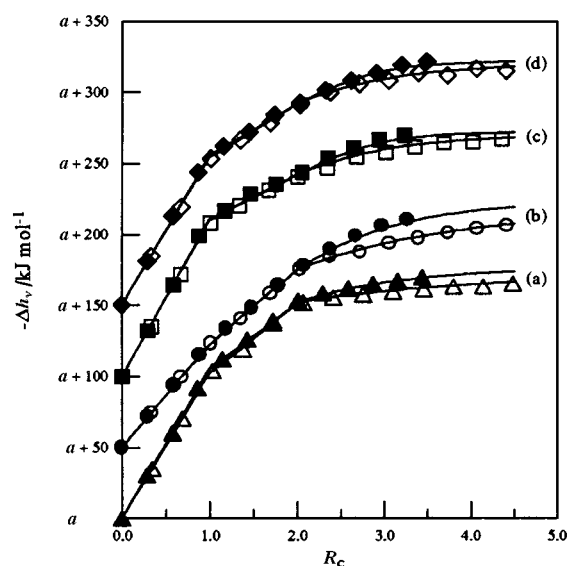
Fig. 3 The total molar enthalpy changes, \Delta h_v , as a function of R_c for silver(I)-P-N systems in pc. (a) a = 0 for \text{Me}_2\text{Npe} : ( \Delta ) 1.985, ( \blacktriangle ) 6.952 \text{mmol dm}^{-3} in \text{Ag}^+ ; (b) a = -50 for \text{Me}_2\text{Npph} : ( \circ ) 2.130, ( \bullet ) 7.011 \text{mmol dm}^{-3} in \text{Ag}^+ ; (c) a = -100 for \text{Me}_2\text{Npp} : ( \square ) 2.015, ( \blacksquare ) 6.853 \text{mmol dm}^{-3} in \text{Ag}^+ ; (d) a = -150 for \text{ppye} : ( \diamond ) 1.913, ( \blacklozenge ) 7.153 \text{mmol dm}^{-3} in \text{Ag}^+ . The solid lines have been calculated from the values of \beta_{m,j} and \Delta H_{m,j}^{\circ} in Table 1.
